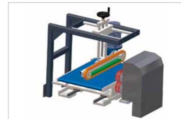
Cinghioi su nastro centro e uscita Overhead sponge conveyors on the central and out feed conveyors of the machine
